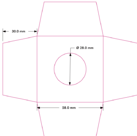
A60下衬: 58x58x30mm
