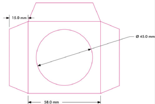
A60上衬: 58x58x15mm
